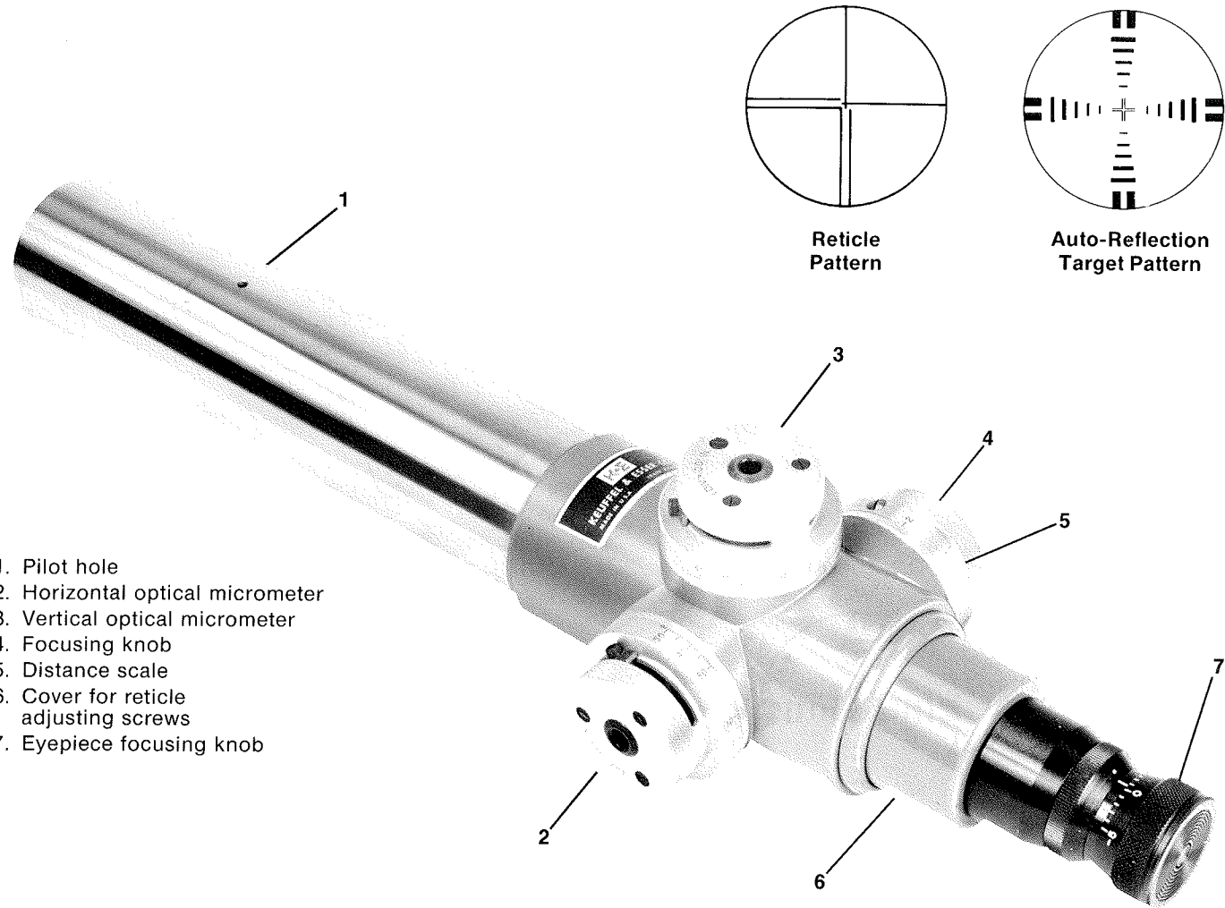
Figure 2-1. 71 2022 Alignment Telescope
