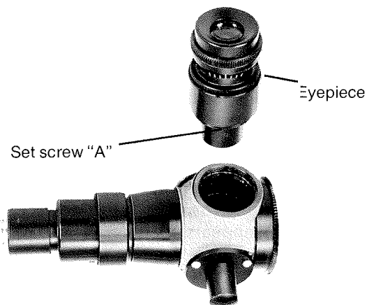
Figure A-5. Installation of Combination Auto-Collimation, Projection, Right-Angle Eyepiece
