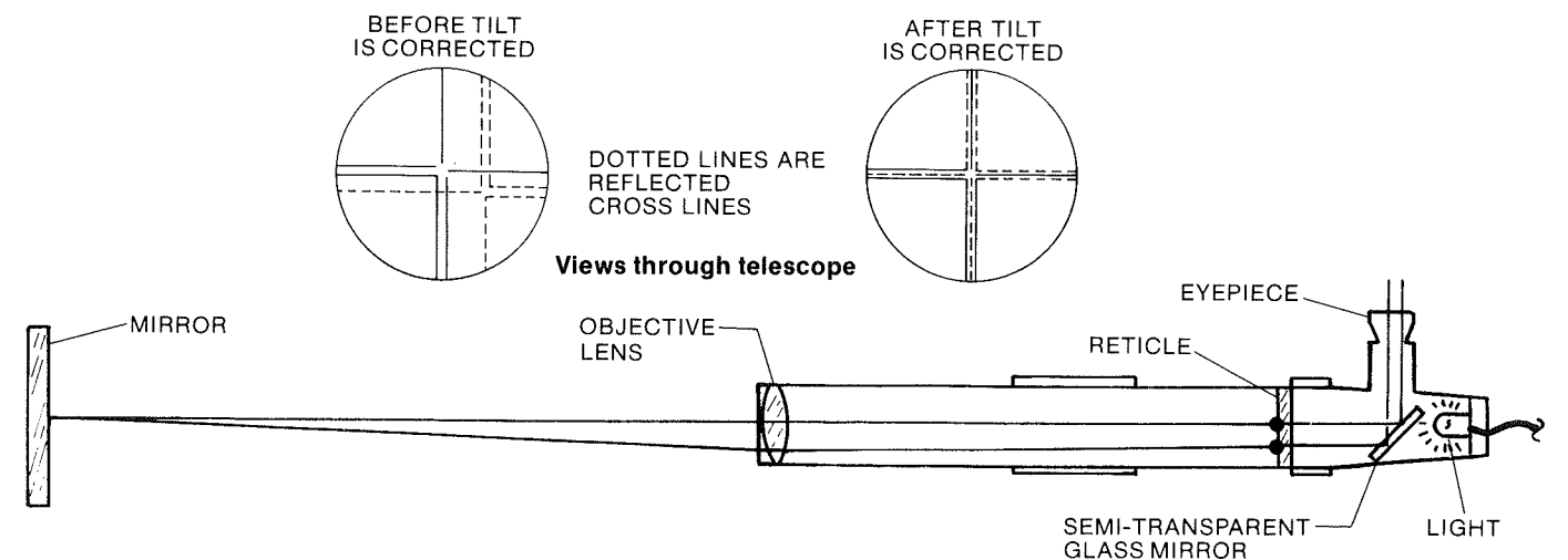
Figure A-3. Auto-Collimation
