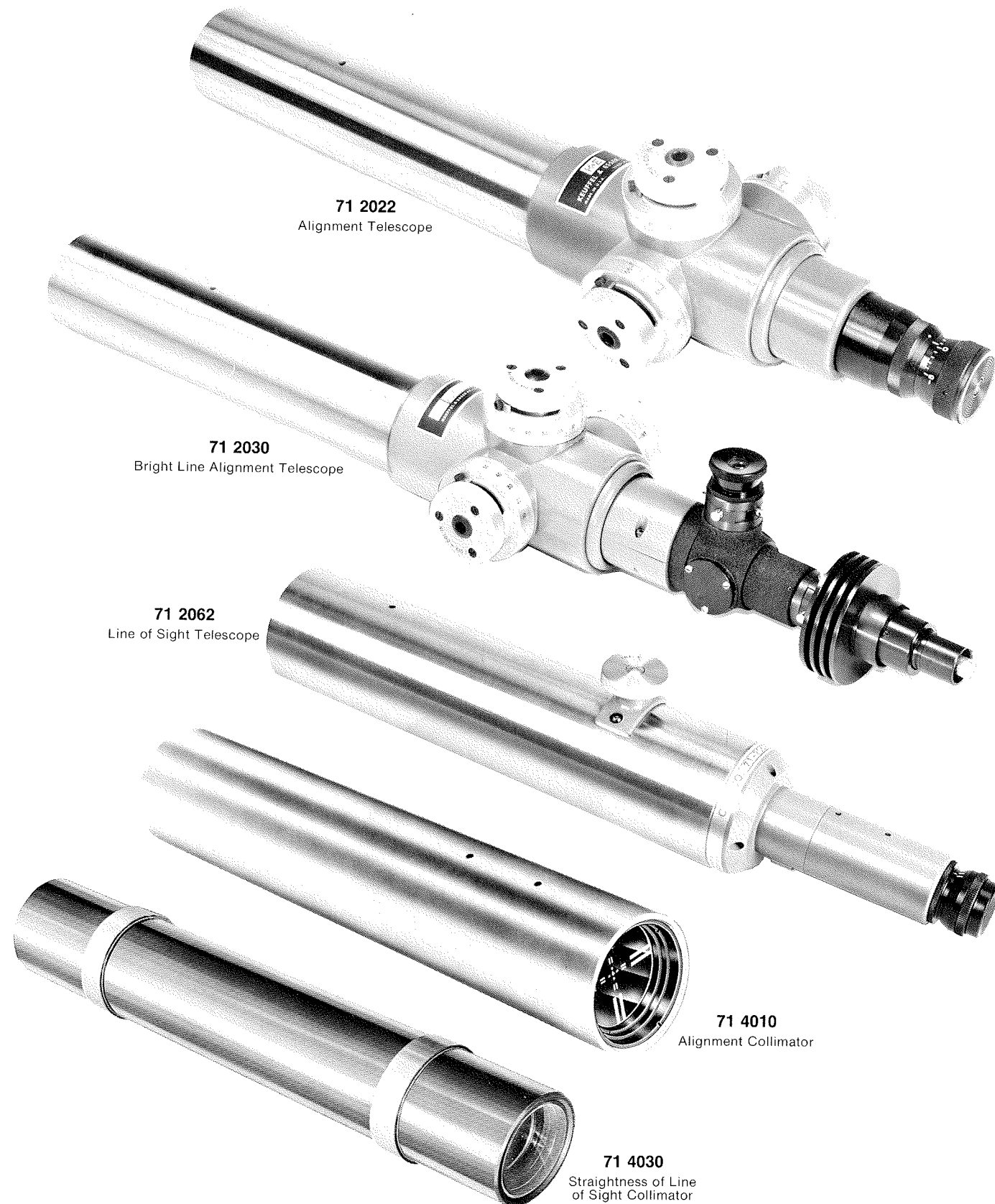
Figure 1-1. Alignment Telescopes, Line of Sight Telescopes and Collimators
