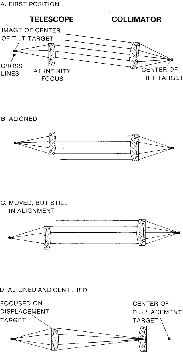
Figure 2-8. Alignment Collimator Used with Alignment Telescope
