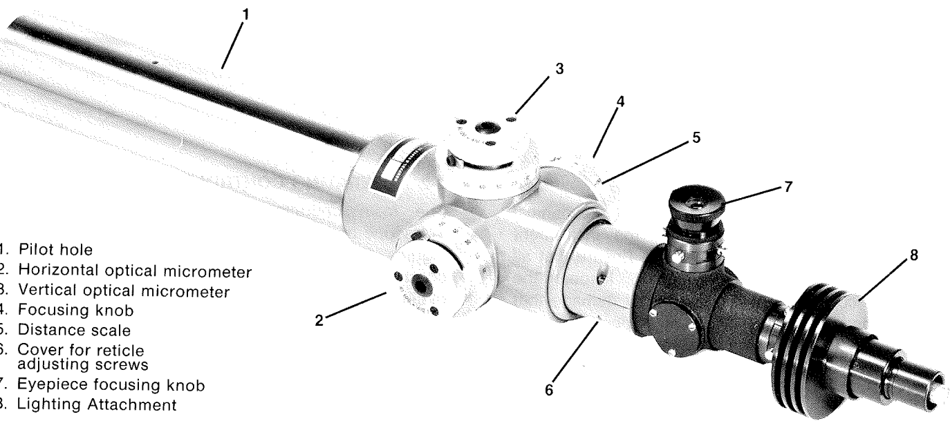
Figure 2-2. 71 2030 Bright Line Alignment Telescope with Lighting Attachment
