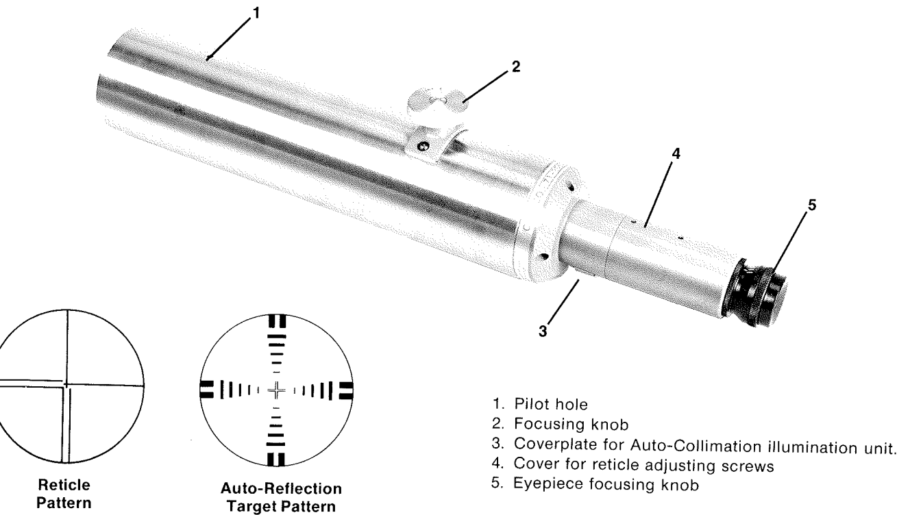
Figure 2-3. 71 2062 Line of Sight Telescope
