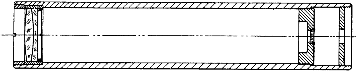
Cross Section of the Alignment Collimator
