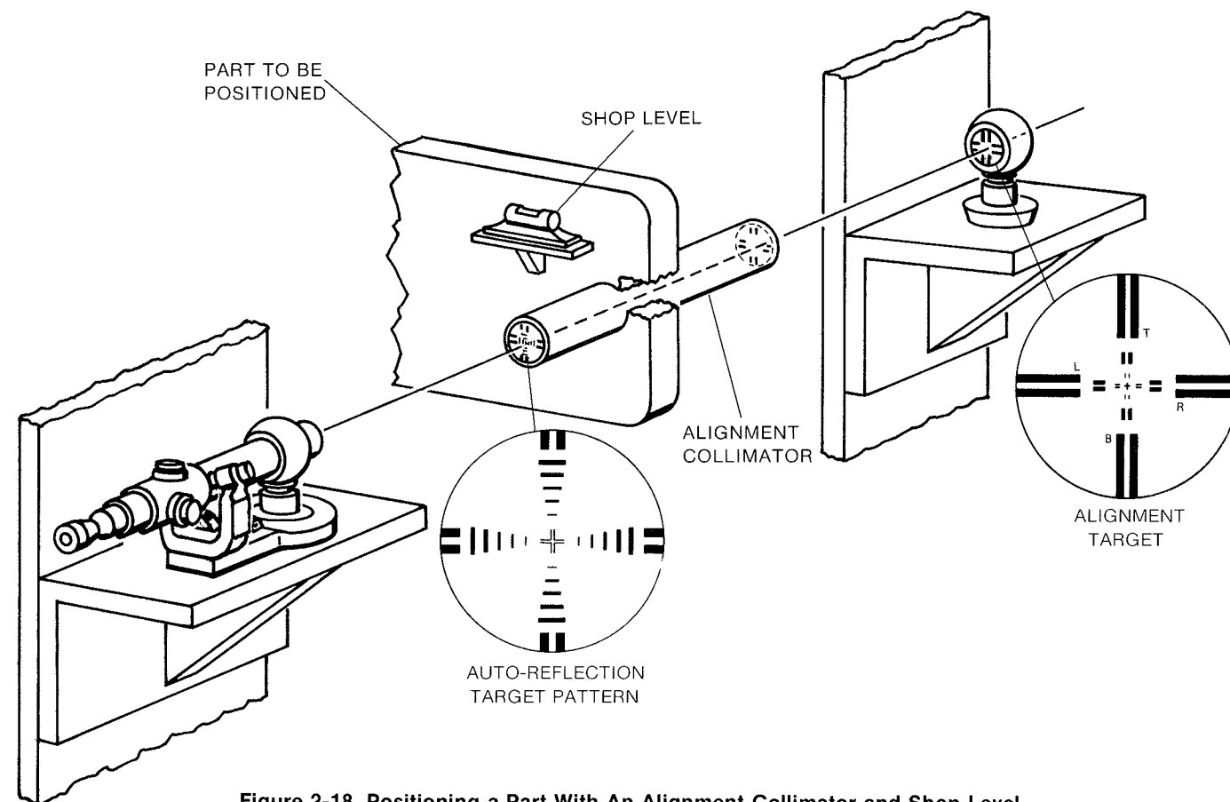
Figure 2-18. Positioning a Part With An Alignment Collimator and Shop Level
