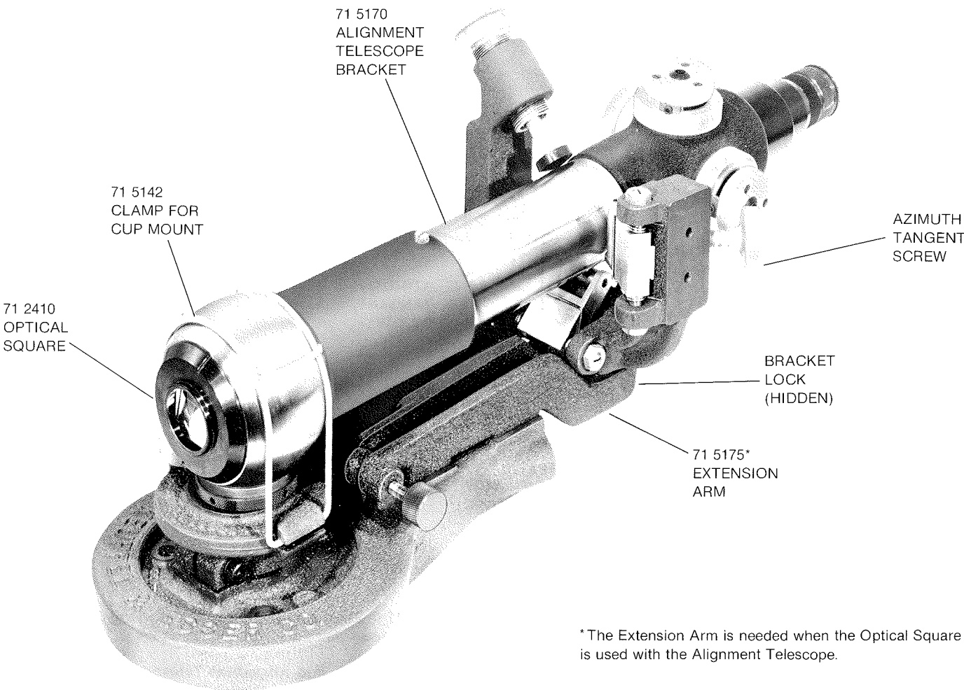
Figure 2-5. 71 5170 Alignment Telescope Bracket
