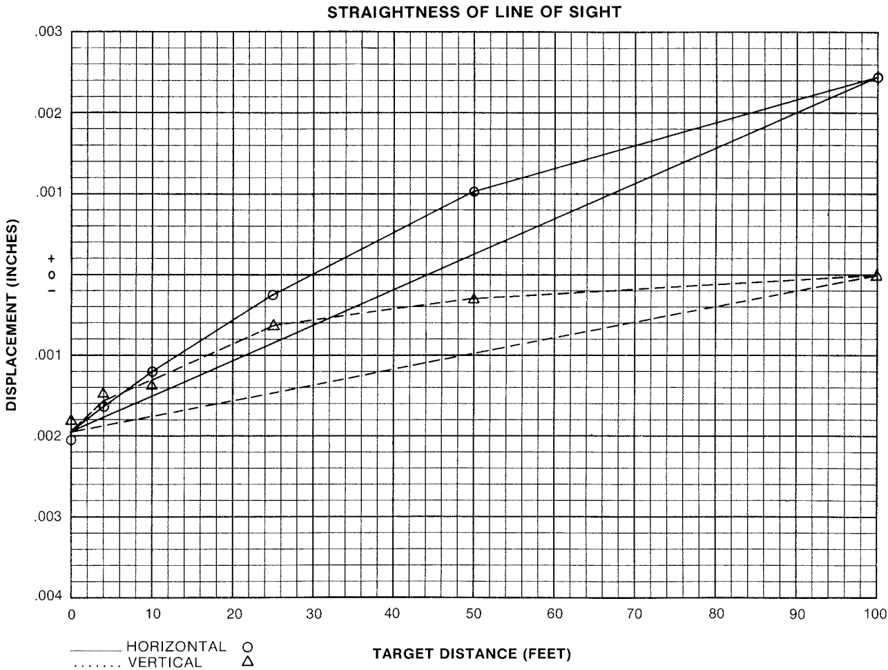
Figure 2-20. Plot of Deviations of Line of Sight
