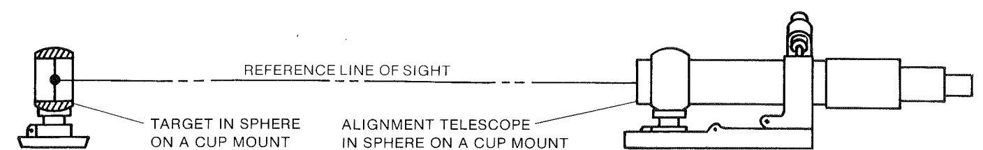
Figure 2-6. Establishing a Reference Line of Sight
