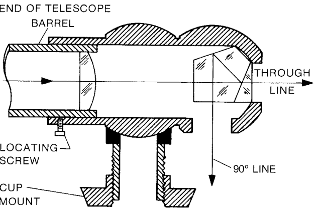
Figure A-7. Schematic View of Double-Sphere Optical Square
