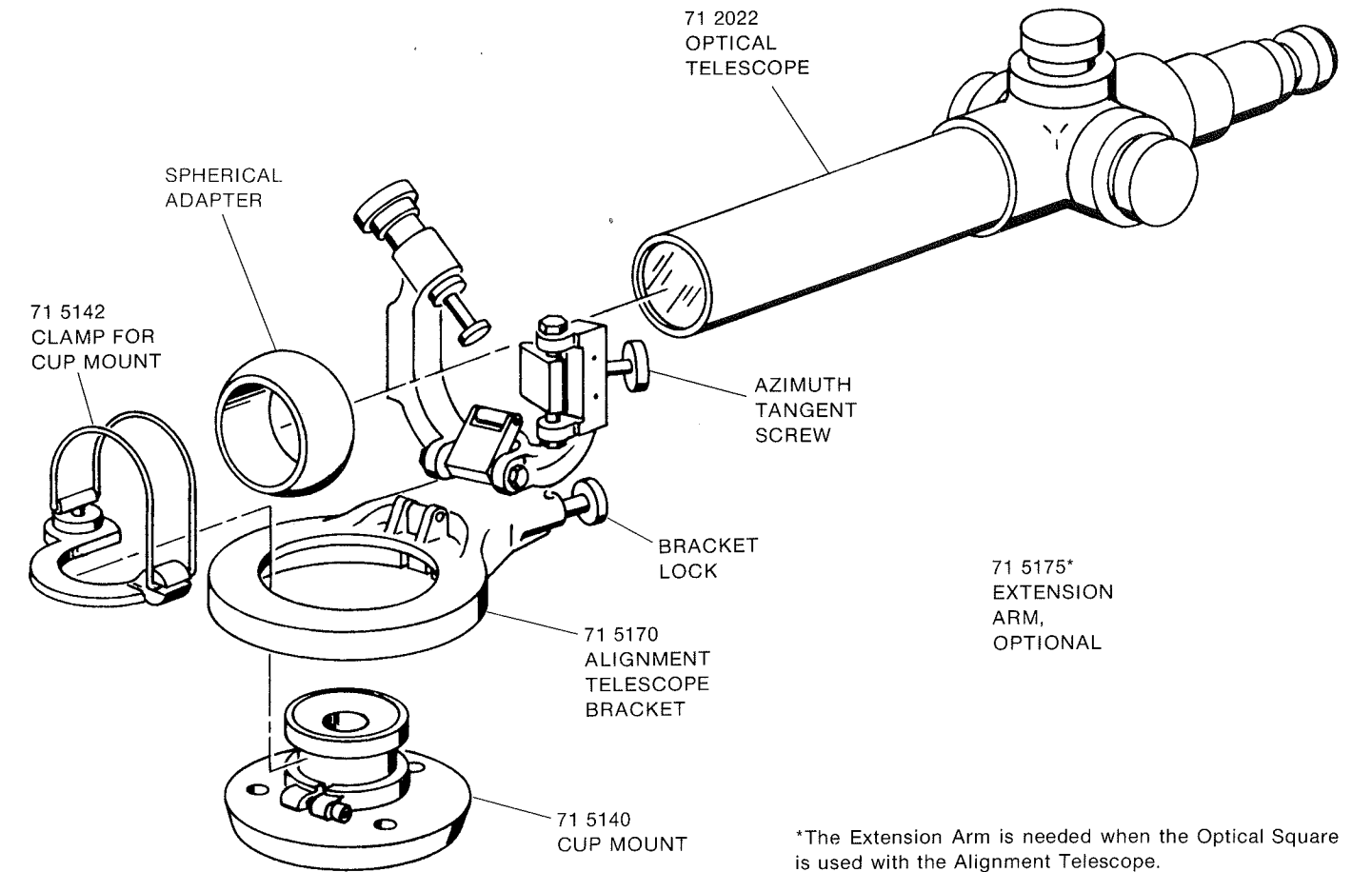
Figure 2-4. Assembly of Cup Mount, Spherical Adapter, Bracket, and Alignment Telescope
